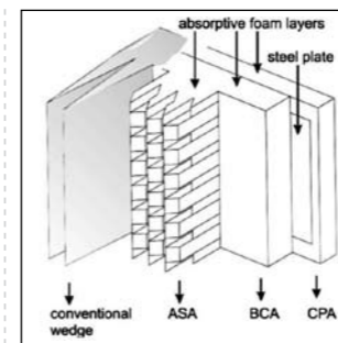
TOP: Mechanical acceptance of acoustic turning vanes at BMWs AAWT ABOVE: The BCA is highly efficient due to its sophisticated structure
